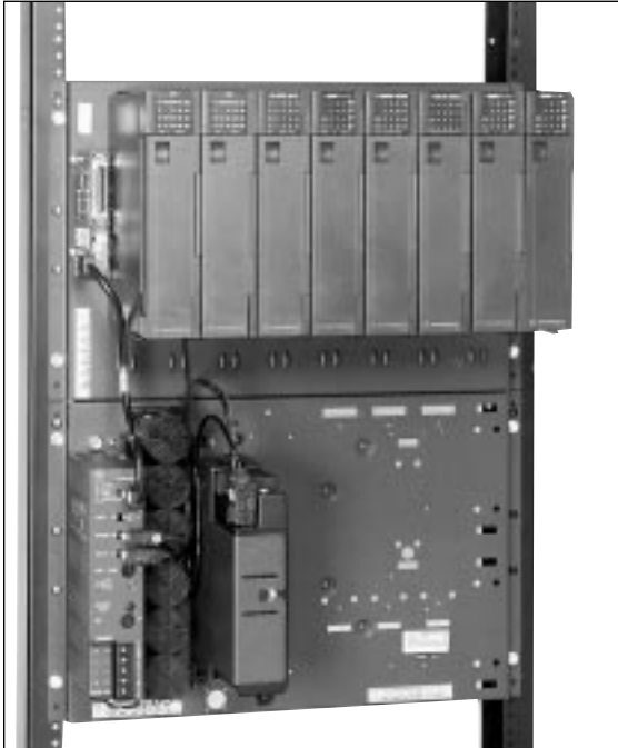
Rackmount with space for 7 I/O modules, expandable to 67
